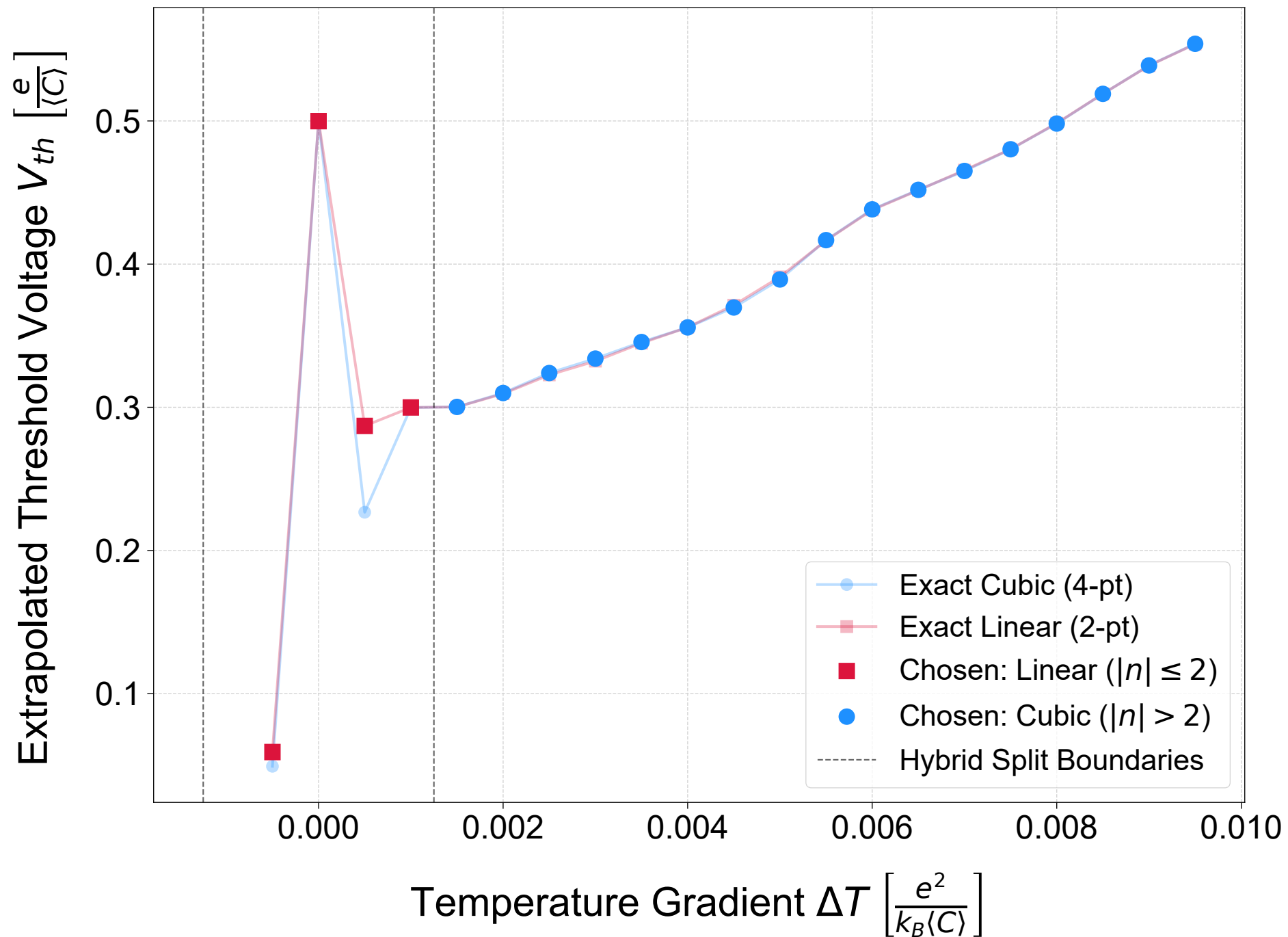
Threshold Voltage V_{th} vs. Gradient \Delta T
